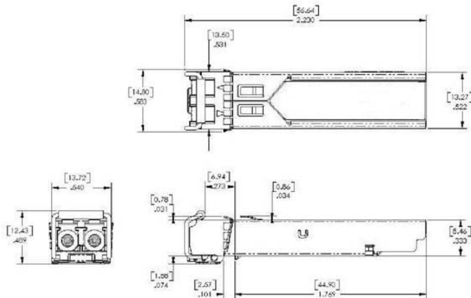
CWDM SFP (dimensions are in inches)
